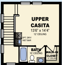
LOWER GUEST CASITA W/ OPTIONAL UPPPER GUEST CASITA ABOVE
