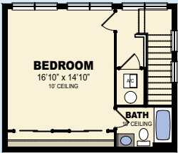
INCLUDED SECOND FLOOR
